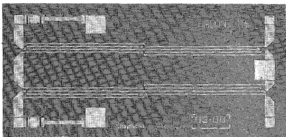
Figure 3. Photograph of the Balun.
